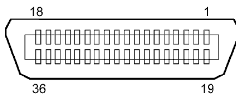
IEEE1284-B-tilkobling
