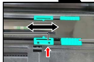
Feed Gap Sensor
