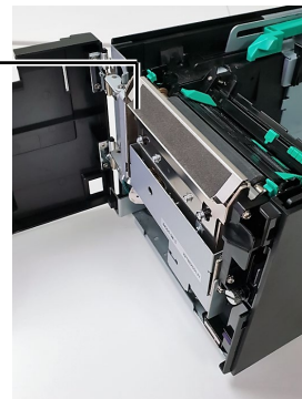
Cutter Module
