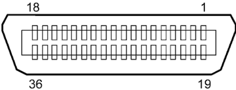
IEEE1284-B Connector
