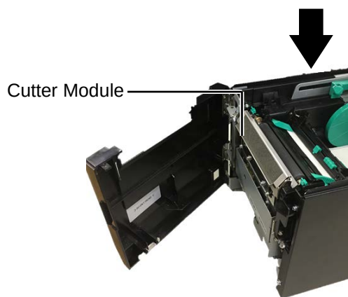
Cutter Module
